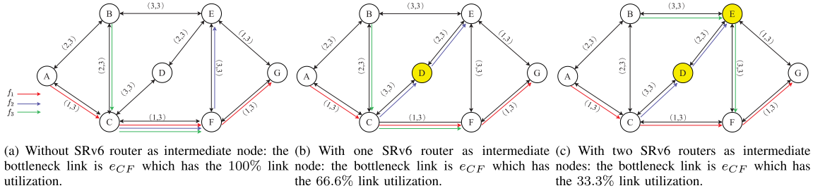
Fig. 4. Three routing solutions with different maximum link utilization using different numbers of SRv6-enable routers. The two-tuple near each edge represents (cost, bandwidth).
