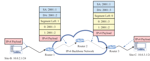
Fig. 2. An example to show interconnection service provided by SRv6. The IPv6 addresses of the three routers are 2001::1, 2001::2 and 2001::3, respectively.
