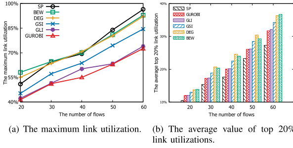
Fig. 14. Small-scale: The impacts of the number of flows on two metrics.
