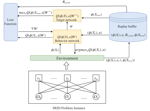
Fig. 10. The framework of Q-learning.
