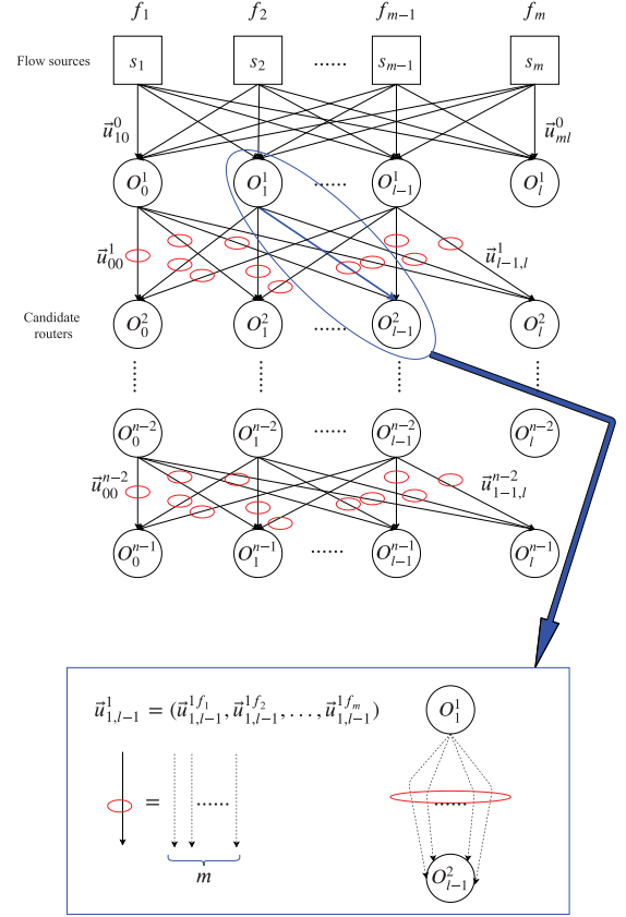
Fig. 19. The multi-level multigraph model for SRID problem.
