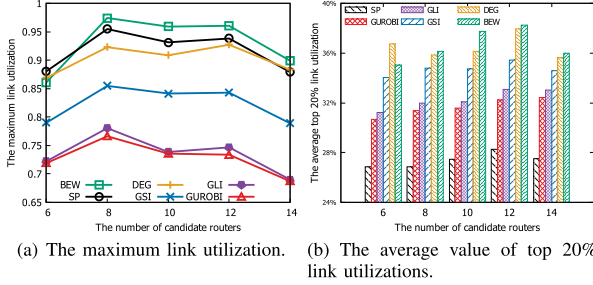
Fig. 15. Small-scale: The impacts of the number of candidate routers on two metrics.
